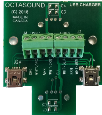
RUSBX2 - LR Long run kit Breakout PC Board.
