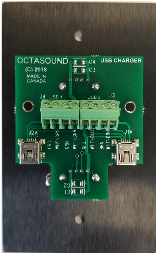
RUSBX2 - Rear View
