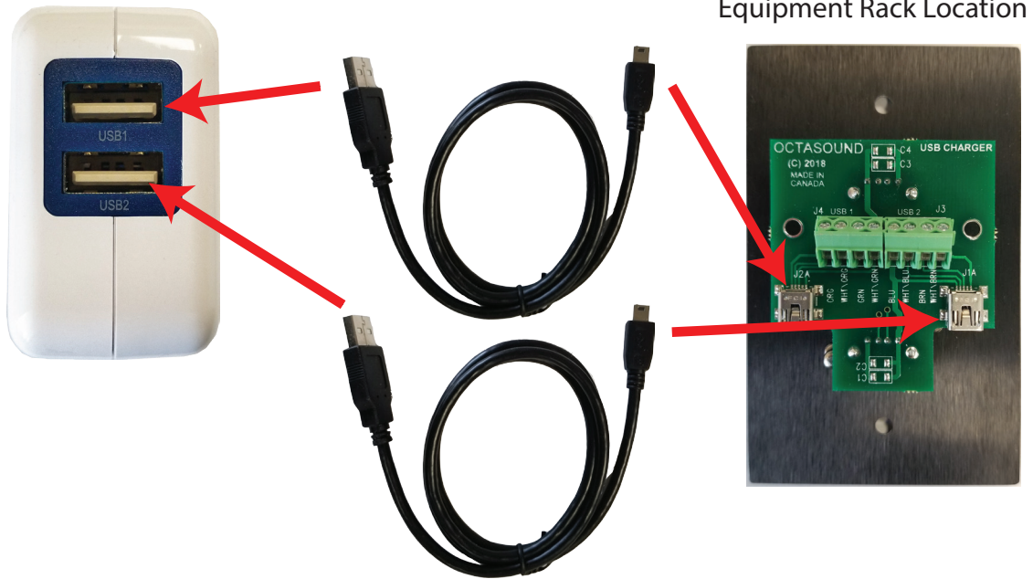
Wiring Diagram RUSBX2-SR Short Run Kit.
