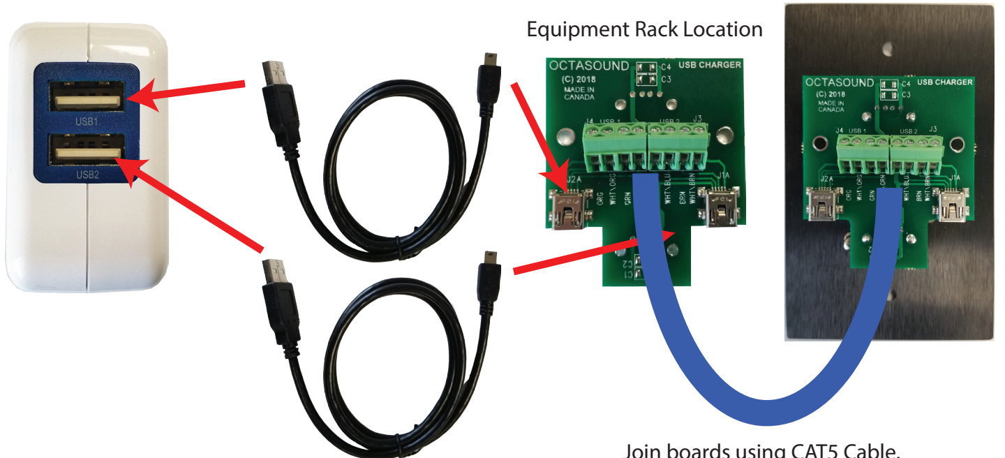
Wiring Diagram RUSBX2 - LR Long Run Kit.
